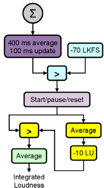
Figure 3 Additional processing in BS1770 rev 2011.
