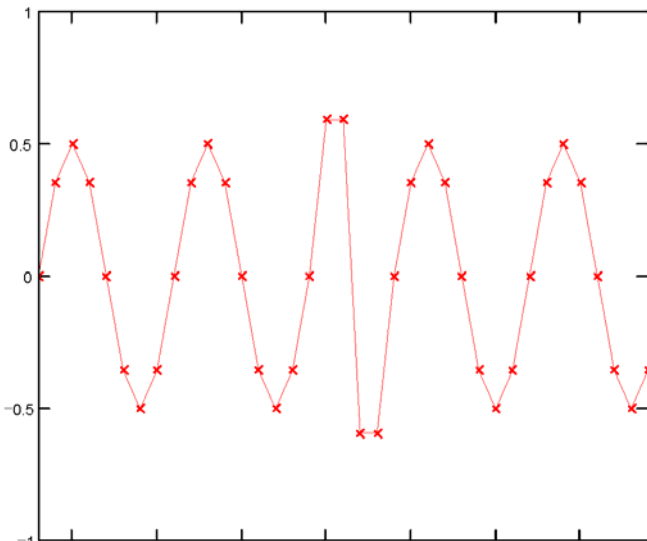
Figure 6a true peak waveform samples
