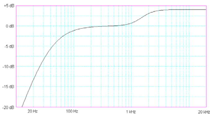
Figure 2 K-weighting filter
